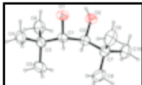
Fig. 1. The molecular structure of the title compound, with atom labels and anisotropic displacement ellipsoids (drawn at 50% probability level) for non-H atoms.
