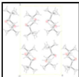
Fig. 3. The packing of the title compound, viewed along [0 0 - 1].
